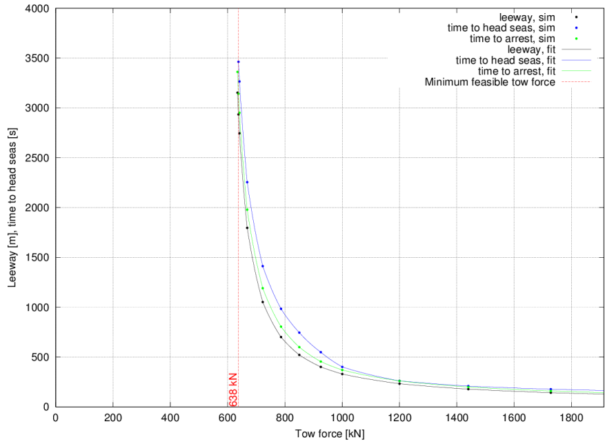
Passenger Ship effect of tow force; 95th percentile environment
