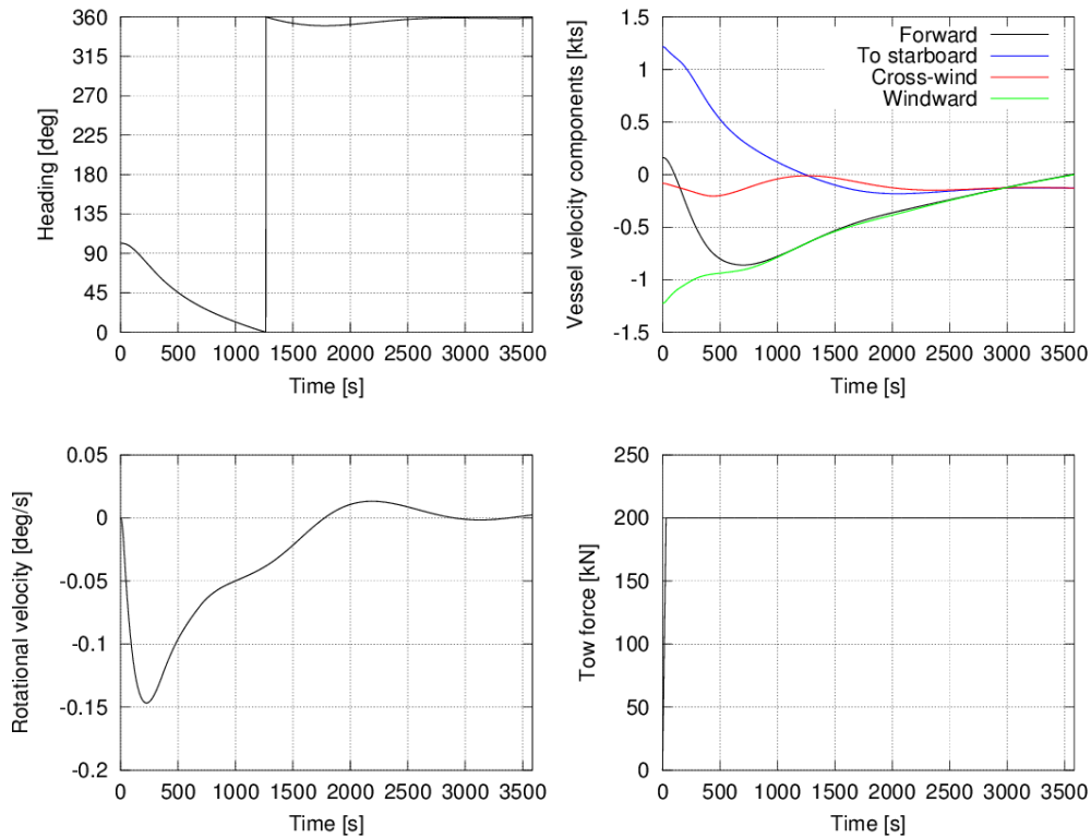
Aframax Tanker, 75th percentile environment, 200 kN pull, port turn
